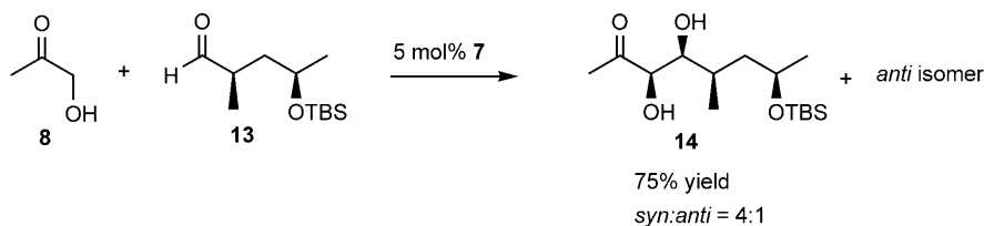
Figure 2. Aldol reaction of aldehyde 13 and hydroxyacetone.
