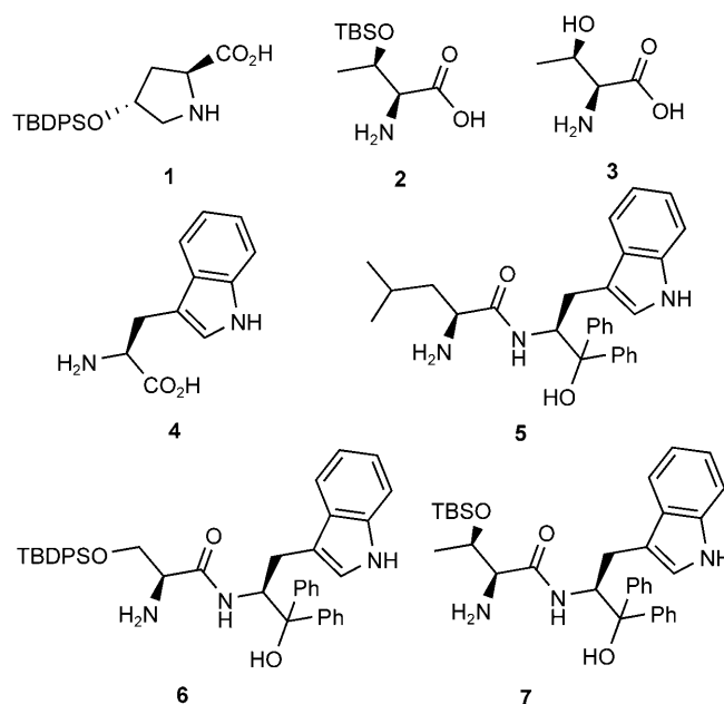
Figure 1. Catalysts screened in the direct aldol reactions.
