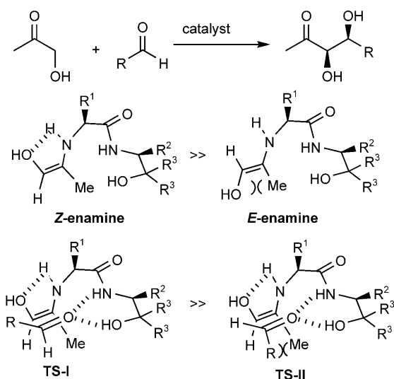
Scheme 2. Plausible transition states in the bifunctional amide-catalyzed aldol reaction of hydroxyacetone.
