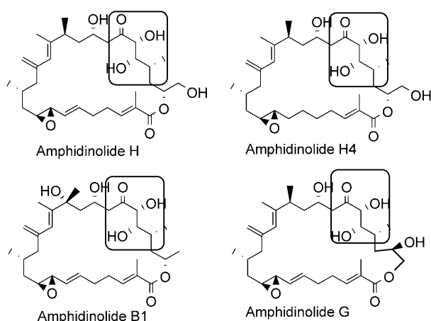
Scheme 1. The \alpha,\beta -dihydroxy ketone unit in amphidinolides.
